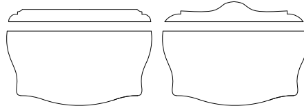
POMA102 L 116/100 P 59 H 2 POMA103 L 116/100 P 59 H 2
