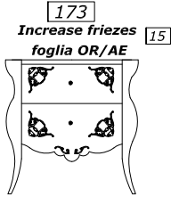
MO 253 L 90/72 P 58 H 83 two big drawers
