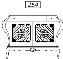
MO 2445 L 132/110 P 60 H 82 two doors two drawers
