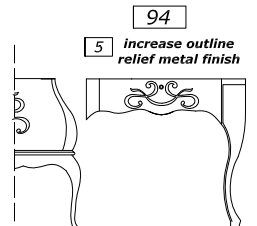
MO 2356 dx L 85 P 48 H 83 one big drawer
